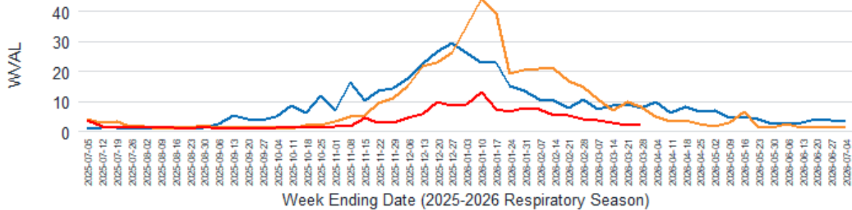
Figure 4. Influenza B Wastewater Concentration Level (WWAL)
